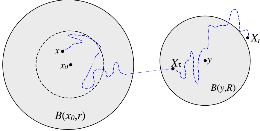
Figure 1: Illustration to (1.8)
