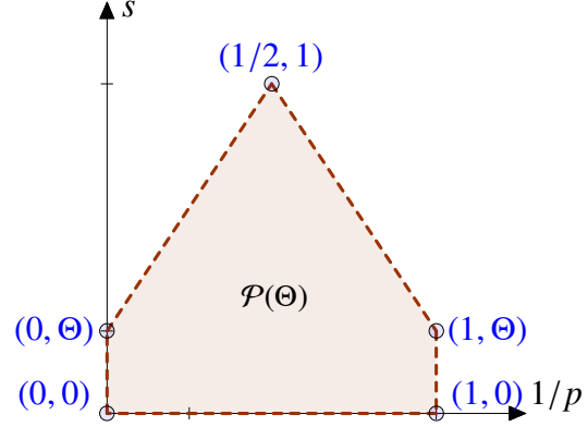
Figure 3: the new range of p and s
