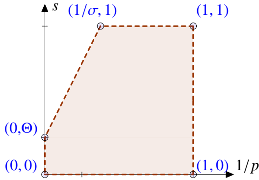
Figure 1: the range for p and s for \mathcal{L} = -\operatorname{div}(A\nabla)
