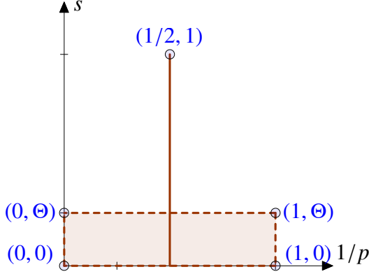
Figure 2: previously known range of p and s
