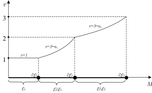
Figure 17: Function v
