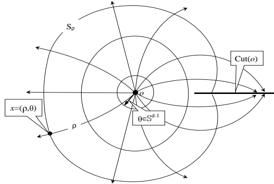
Figure 3: Polar coordinates in M \setminus Cut^*(o)
