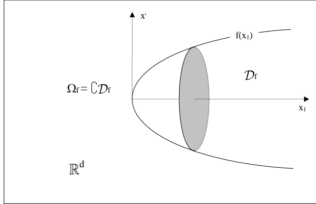
Figure 9: Set \Omega_f is the exterior of the domain of revolution \mathcal{D}_f .
