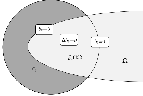
Figure 10: Function b_k
