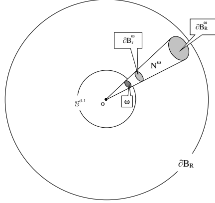
Figure 24: Capacitor (B_r^\omega, B_R^\omega) in N^\omega
