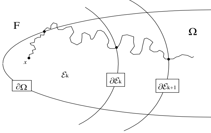
Figure 13: Events \mathcal{A}_k and \mathcal{A}_{k+1}
