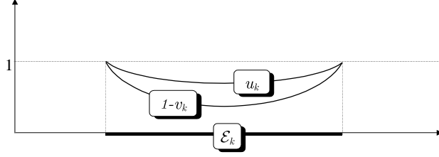
Figure 16: Functions u_k and 1 - v_k
