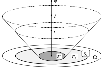
Figure 20: Function \psi and sets E_t, S_t
