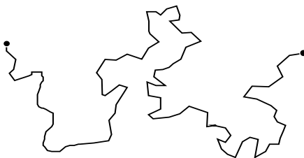
Figure 2: The Brownian motion on \mathbb{R}^2
