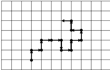
Figure 1: The random walk on \mathbb{Z}^2
