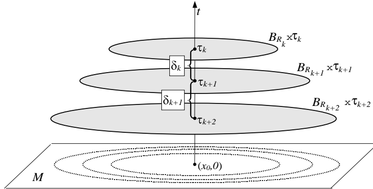
Figure 21: Sequences \tau_k, \delta_k and B_{R_k}
