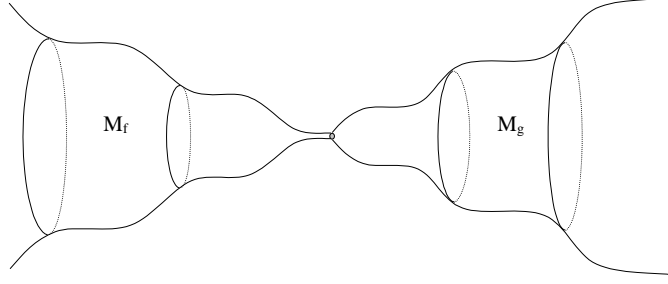
Figure 19: Connected sum of M_f and M_g
