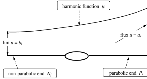
Figure 30: Limits and fluxes of a harmonic function u
