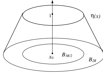
Figure 22: Function \eta(x)
