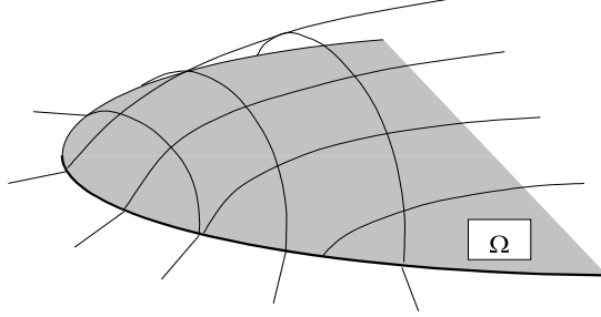
Figure 8: Admissible subharmonic function v for \Omega .
