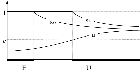
Figure 14: Functions s_\Omega , s_U and u
