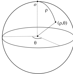
Figure 5: The polar coordinates on \mathbb{S}^2
