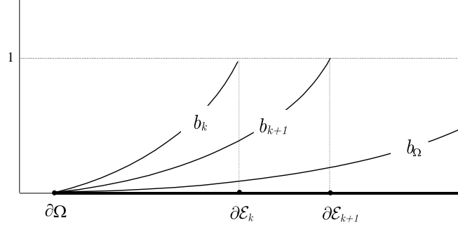
Figure 11: Sequence of b_k
