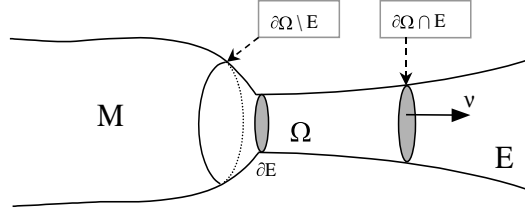
Figure 29: Flux of u on the end E
