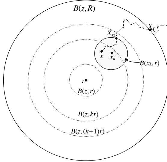
Figure 4: Exit times from B(x_k, r) and B(z, R)
