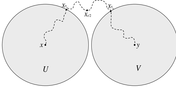
Figure 5: Illustration to (4.14)
