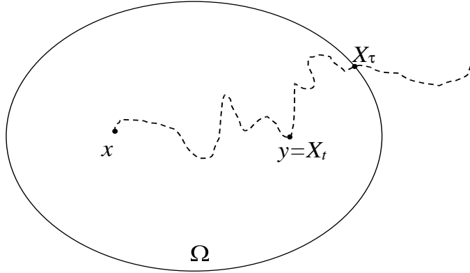
Figure 3: Illustration to the proof of Lemma 3.12
