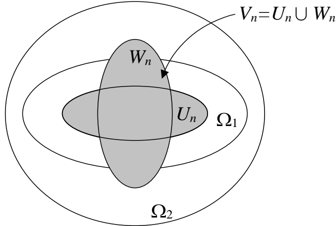
Figure 1: Sets U_n, W_n, V_n
