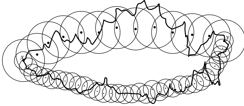
Figure 8: Two shortest chains of \varepsilon -balls for two distinct values of \varepsilon provide different routes for the diffusion from x to y for two distinct values of time t .
