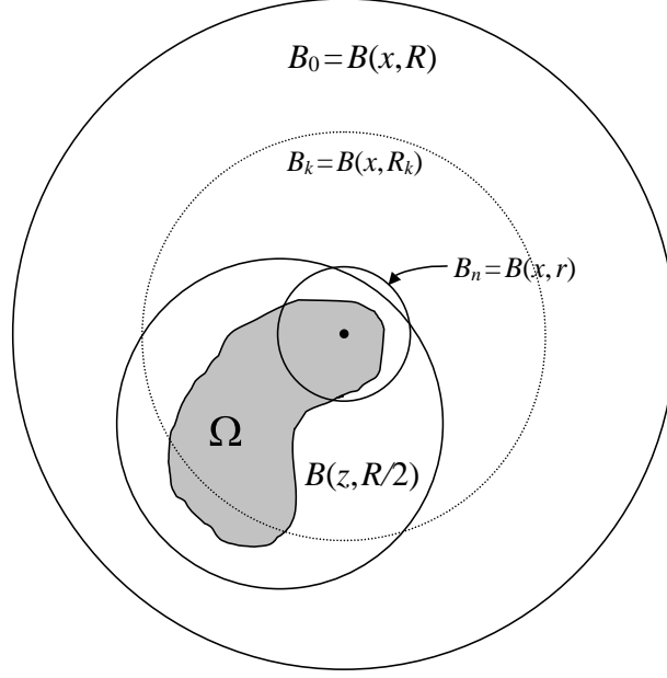
Figure 2: Balls B_k
