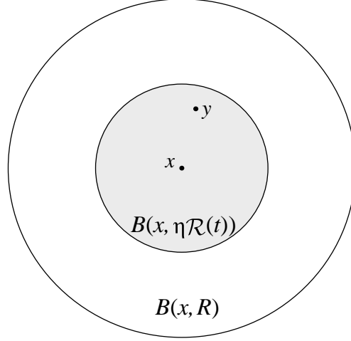
Figure 6: Illustration to Theorem 5.14
