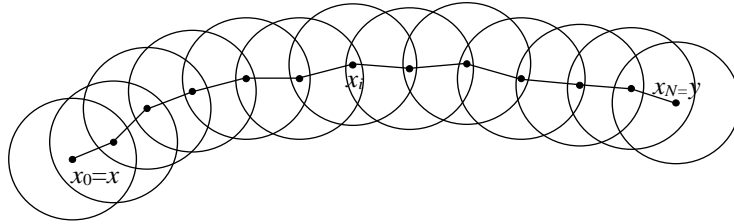
Figure 7: An \varepsilon -chain connecting x and y
