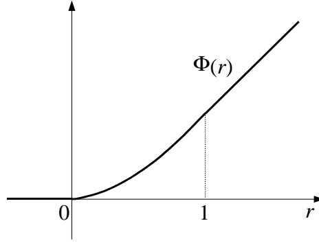
FIGURE 5. Function \Phi(r)
