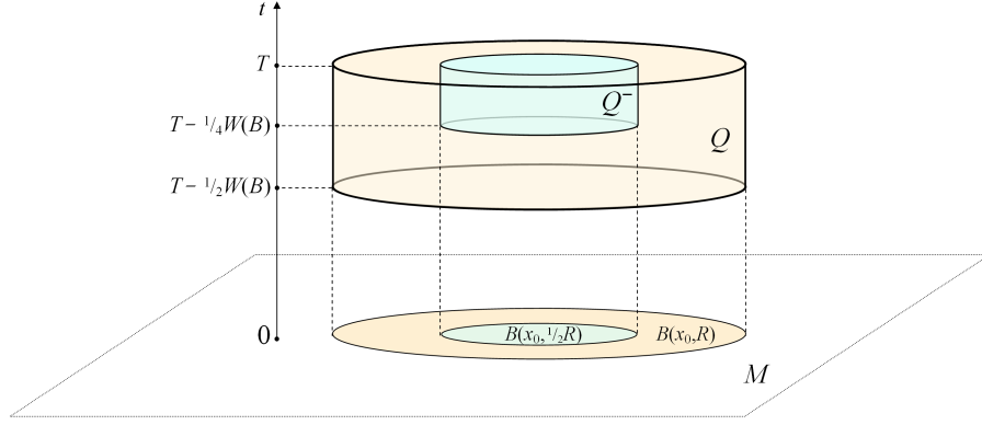
FIGURE 2. Cylinders Q^- and Q
