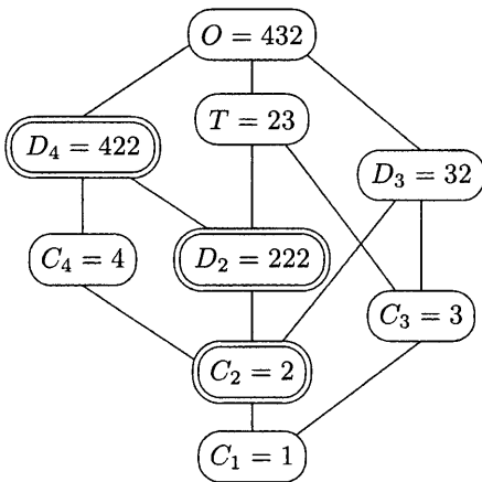
Fig. 1. Subgroups of 432. Single circles are used if all subgroups of one type are conjugate under operations of 432, double circles indicate that the subgroups of these types are divided into two classes of conjugate subgroups. For instance, there exist nine different subgroups of type 2 corresponding to the nine rotations 2 of 432. Three of them are rotations about the cubic fourfold axes and the other ones are rotations about the cubic twofold axes. The fourfold axes are crystallographically equivalent directions, and so are the six twofold axes. Correspondingly we have two classes of conjugate subgroups of type 2, one class consisting of three subgroups and the other one consisting of six subgroups.
