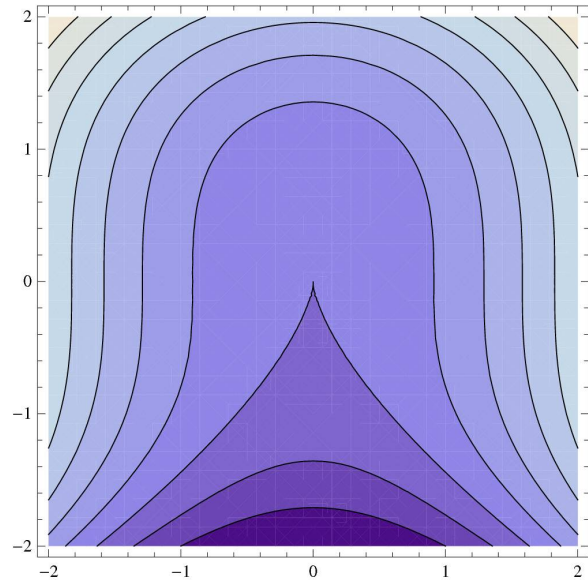
Figure 3: f(x, y) = 3x^2 + y^3
