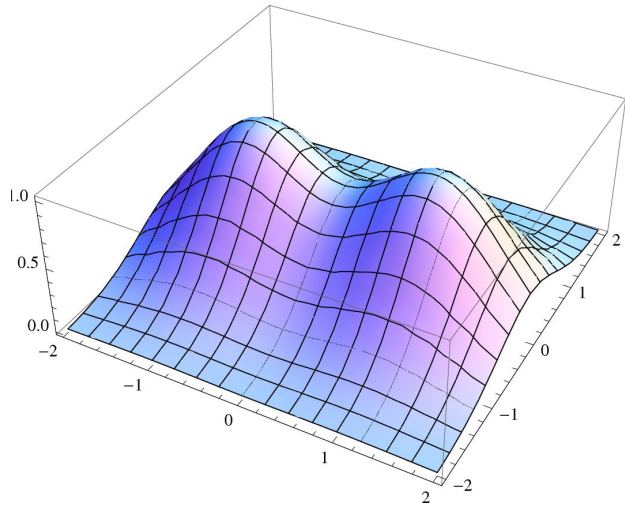
Figure 1: f(x, y) = e^{-(x-1)^2 - y^2} + e^{-(x+1)^2 - y^2}
