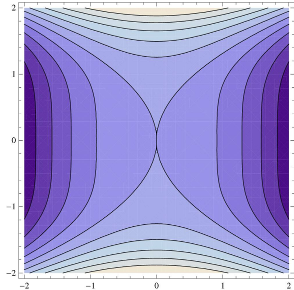
Figure 2: f(x, y) = -3x^2 + y^4
