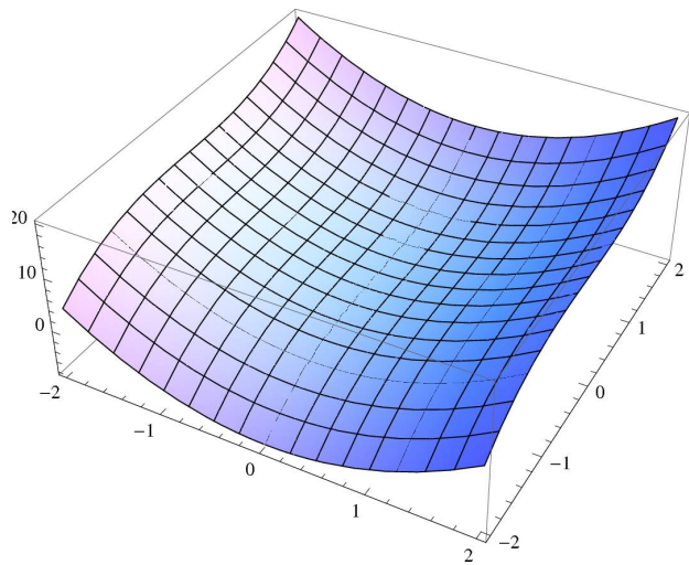
Figure 3: f(x, y) = 3x^2 + y^3
