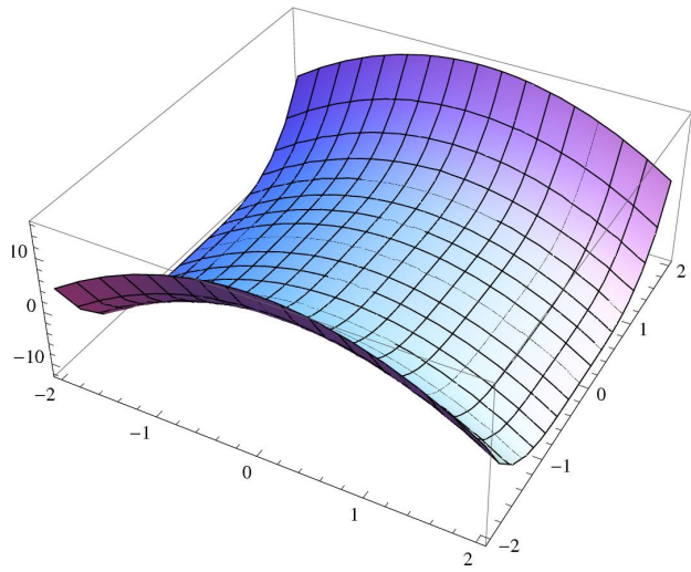
Figure 2: f(x, y) = -3x^2 + y^4
