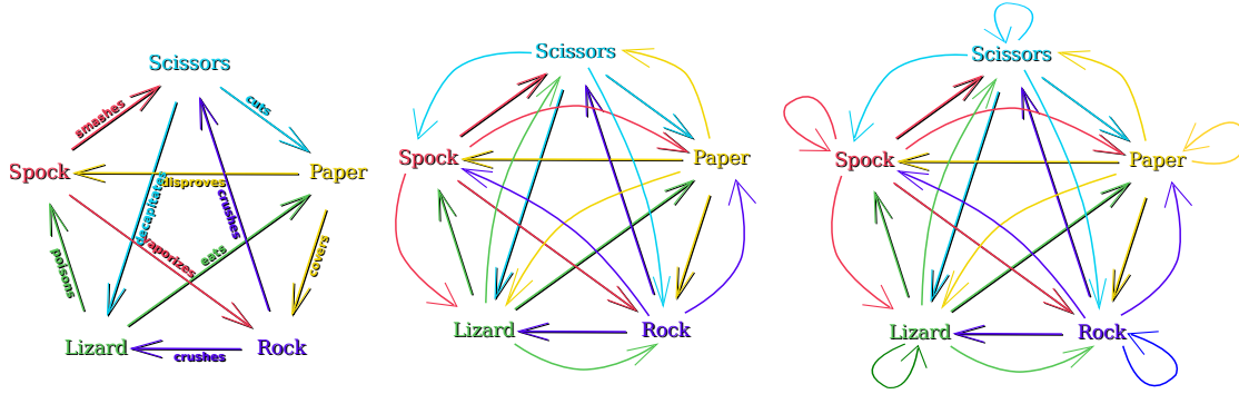
Figure 2: A relation (W, R) (left), its second iterate (W, R^2) (middle) and (W, R^3) (right).
