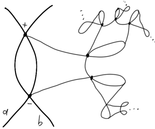
Figure 43: Building a Casson handle.
