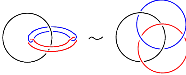
Figure 56: A symmetry of the Borromean rings
