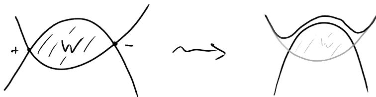
Figure 35: The Whitney trick in the plane.
