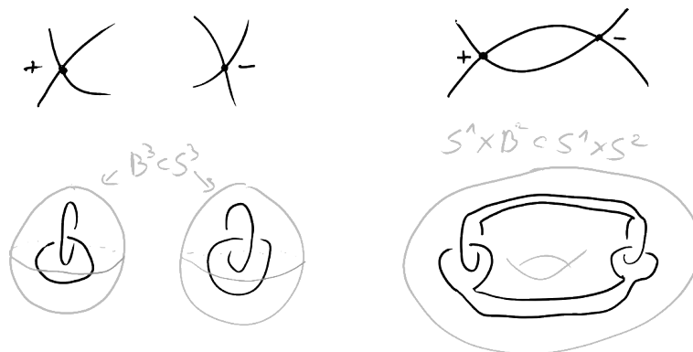
Figure 37: From two Hopf links to a Bing double
