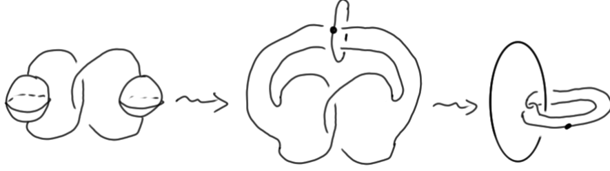
Figure 47: Kirby diagrams of a single (negative) self-plumbing of D^2 \times D^2 .
