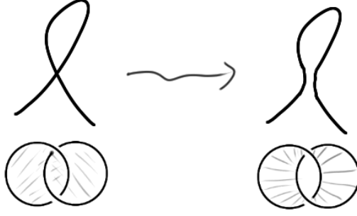
Figure 63: Resolving double points of surfaces.
