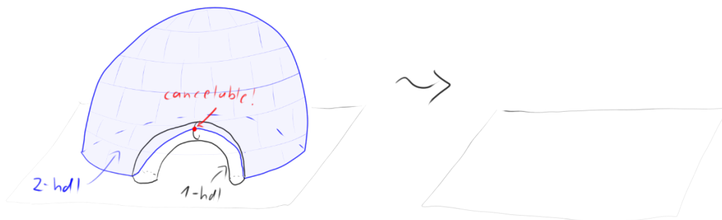
Figure 59: An igloo melting back into the arctic.
