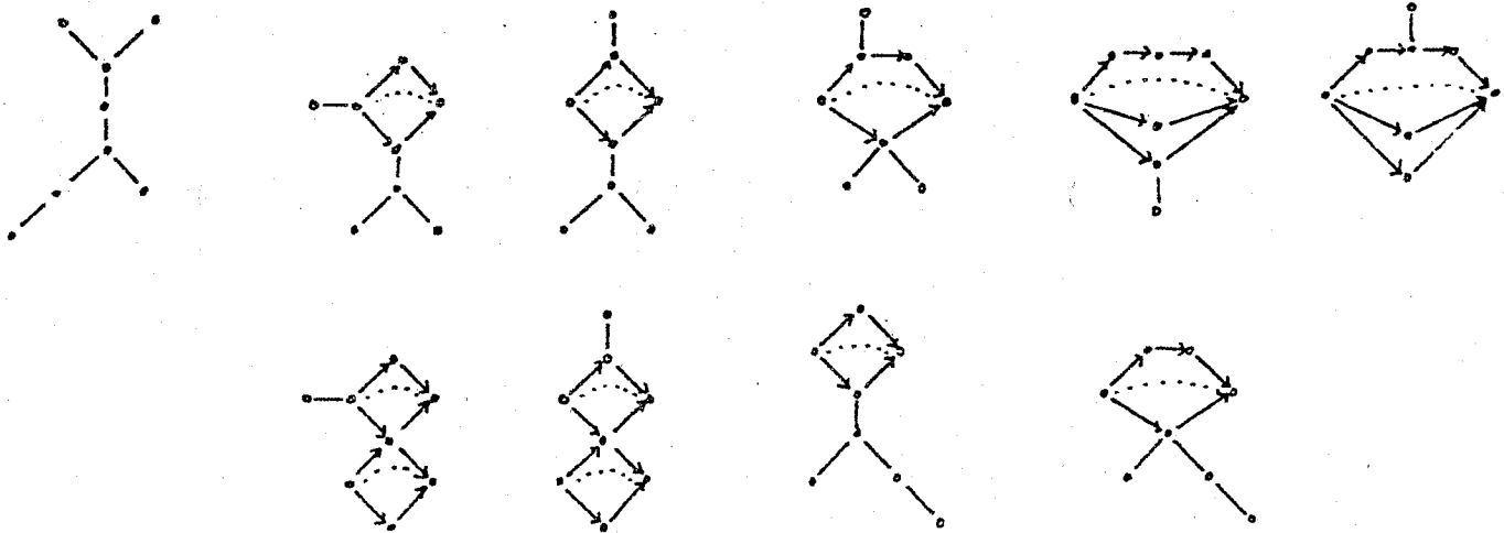
The frames of type \tilde{D}_7
