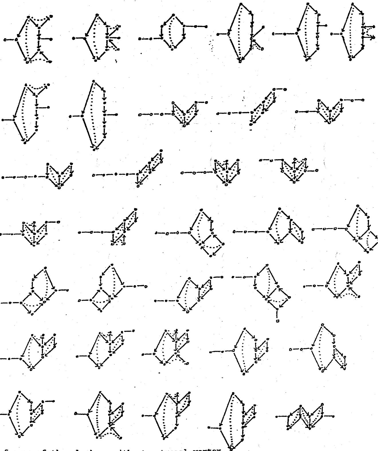
The frames of the algebras without extremal vertex
