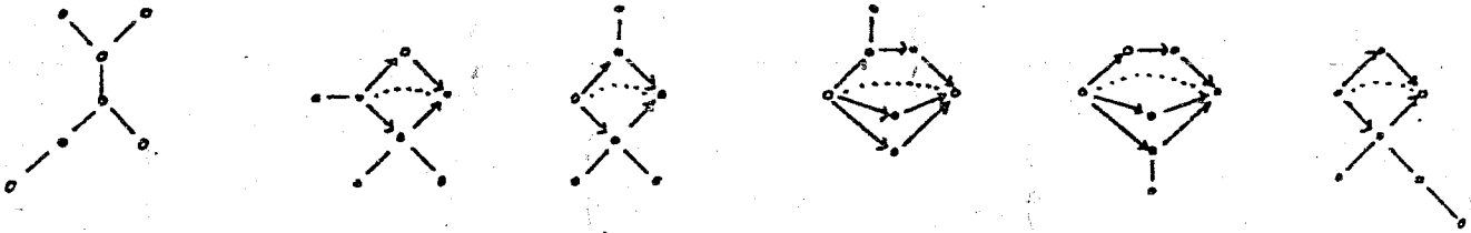
The frames of type \tilde{D}_6
