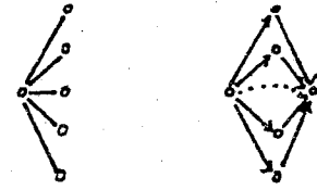
The frames of type T_{11111}
