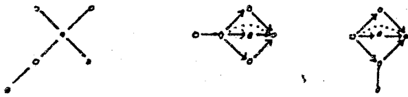
The frames of type \tilde{D}_5
