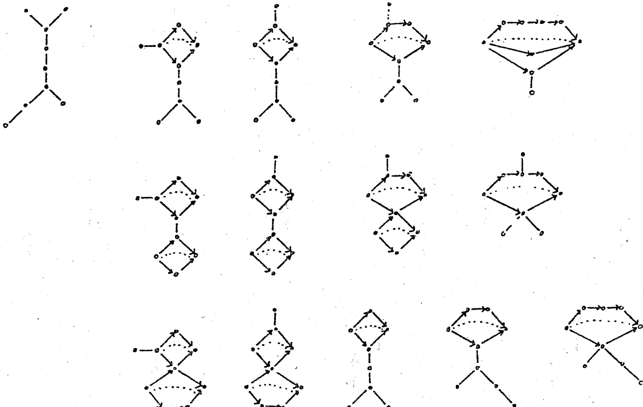
The frames of type \tilde{D}_7
