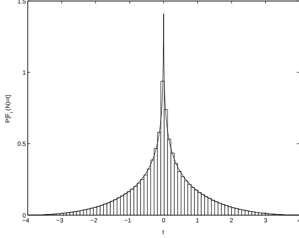
FIGURE 2. Scaled distribution of normalized matrix elements F_i(\vec{n}) = N \langle T_N(\vec{n}) \phi_i, \phi_i \rangle , \vec{n} = (1, 1, 0, 0) \notin Z_1 \cup Z_2 for N = 1613 . Plotted together the corresponding distribution y(t) = \frac{1}{2\pi^2} \int_{t/2}^2 \sqrt{(4 - s^2)(4 - (\frac{s}{t})^2)} \frac{ds}{s}
